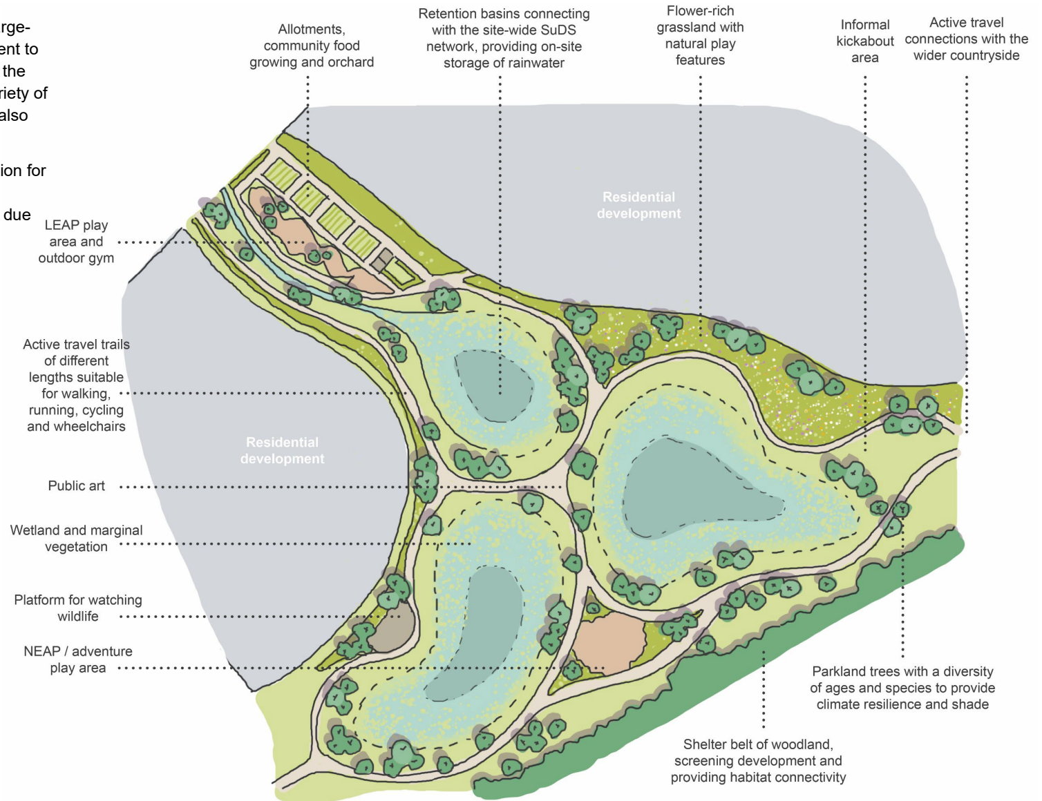
Figure 10: How large-scale retention basins can be incorporated into the design of residential schemes.
