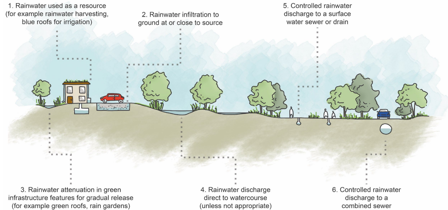
Figure 9: The Drainage Hierarchy.
